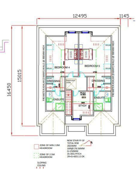
Proposed Second Floor
